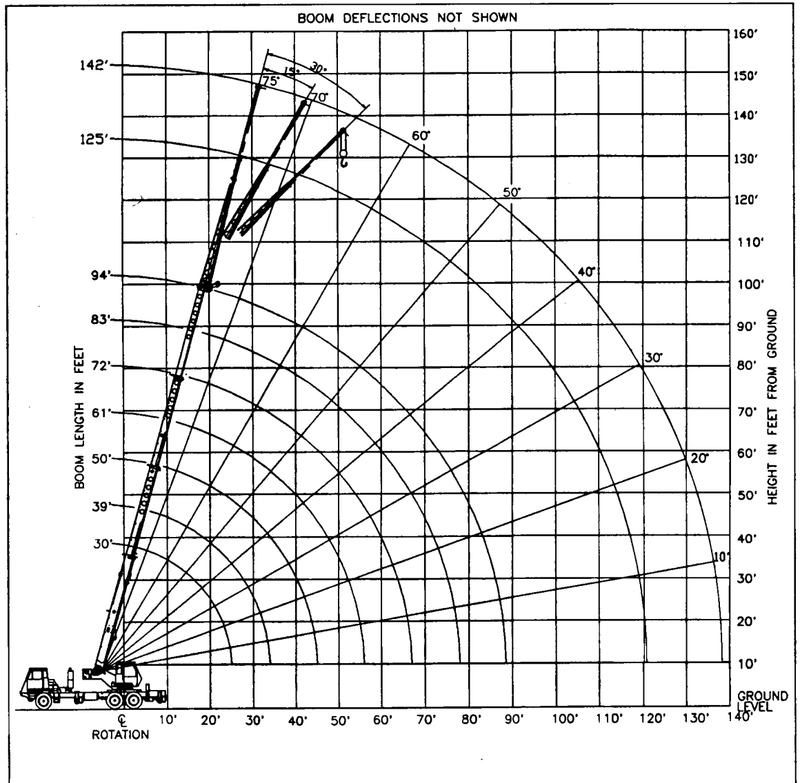
Range Diagram (30' - 94' boom)
